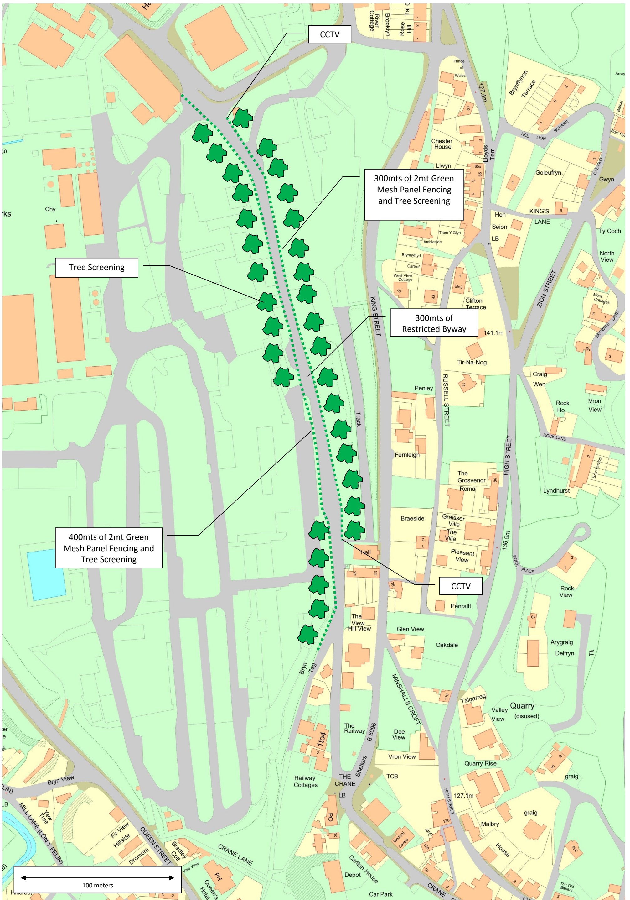
Eastman's section of Jessop's Tramway 300mts Plan
